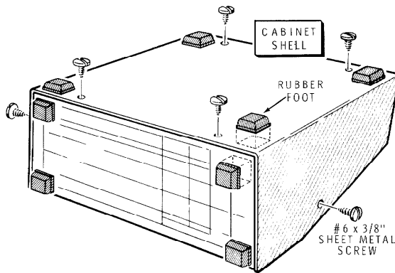
PICTORIAL 16
