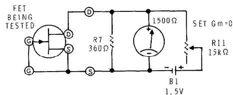
Gm Figure 13
