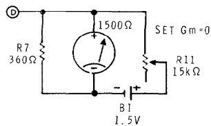
Gm = 0 Figure 12
